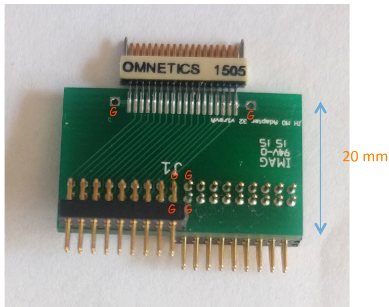
Adapter Millmax16_Omnetics 32
